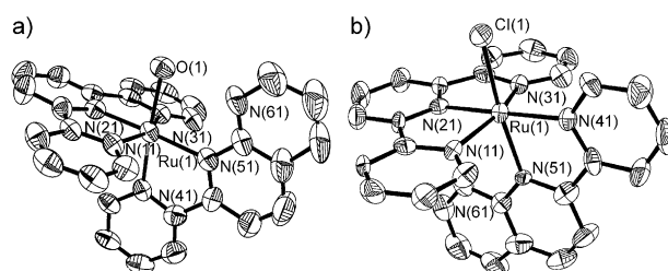
Figure 1. The molecular structures of cations a) [\mathbf{1}(\text{OH}_2)]\text{Cl}_2 and b) [\mathbf{2}(\text{Cl})](\text{PF}_6)_2 .
